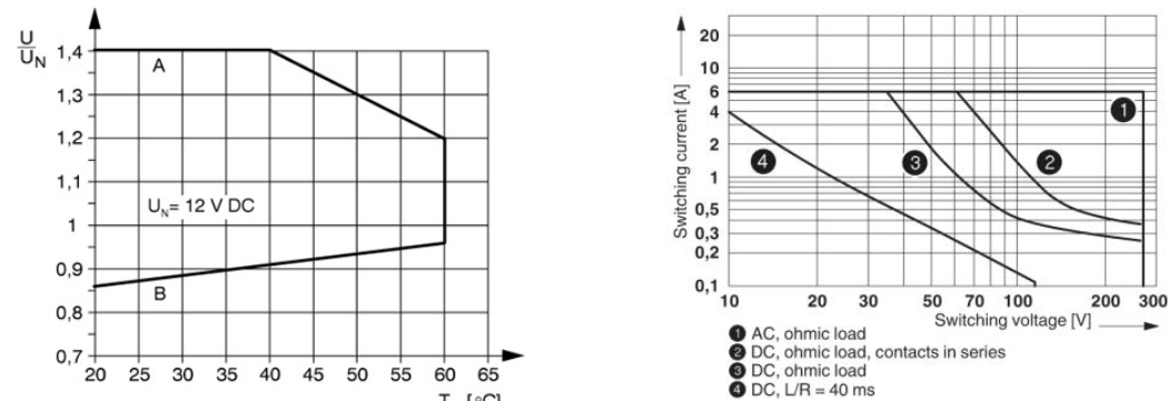
Interrupting rating
