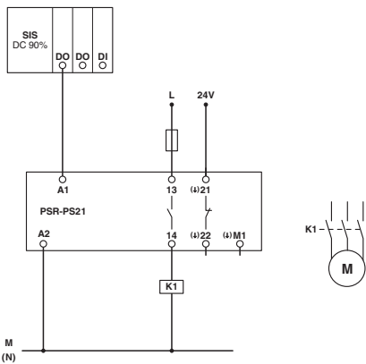
Circuit diagram
