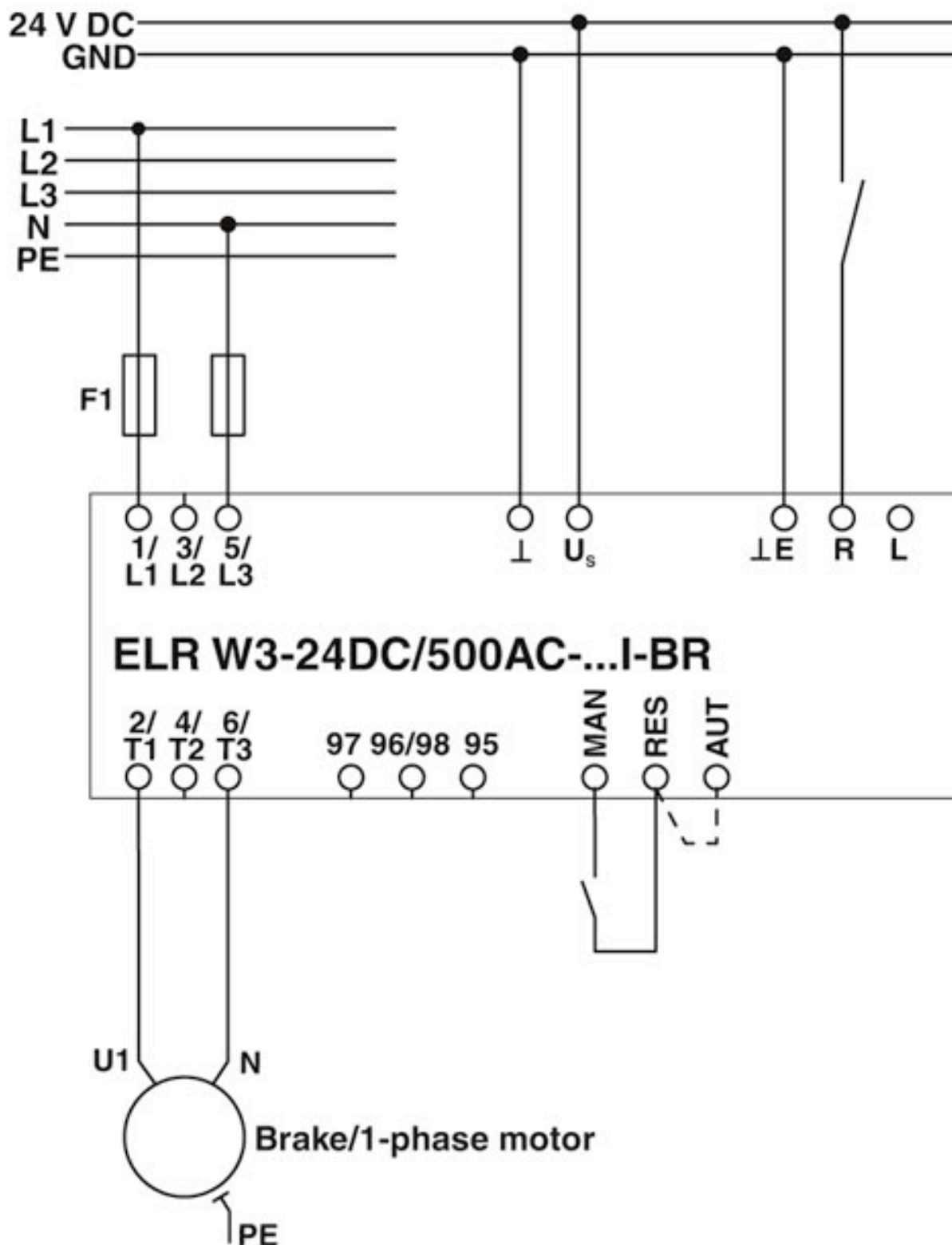
Circuit diagram
