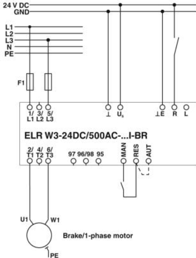
Circuit diagram
