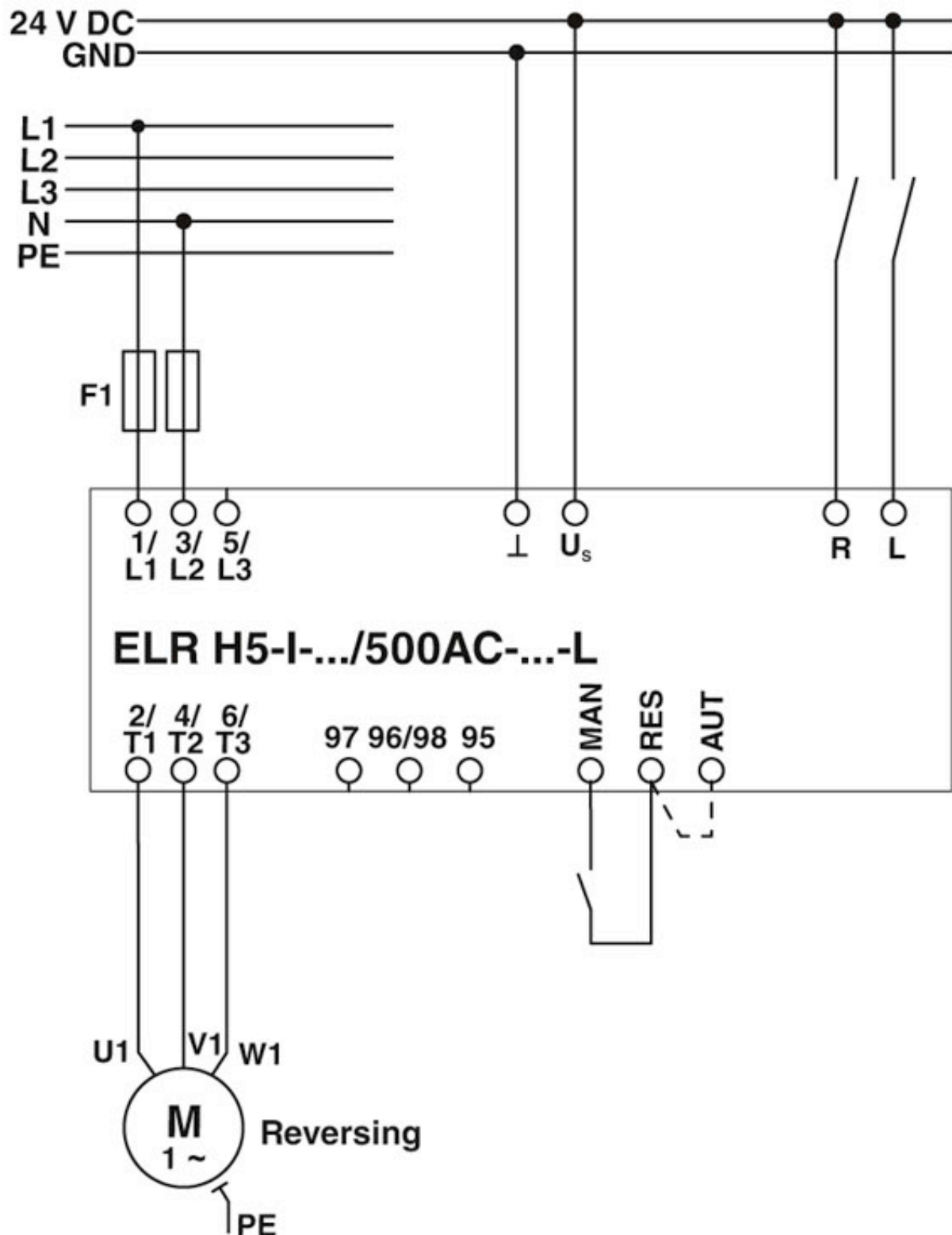
Circuit diagram
