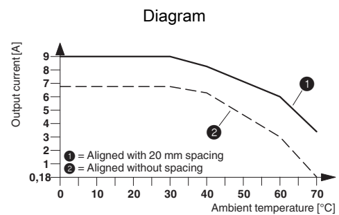
Derating curve for ELR H5-SC-24DC/500AC-9 100% operating time
