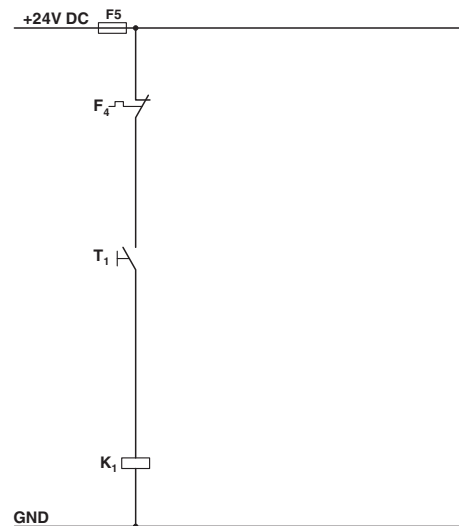
Circuit diagram
