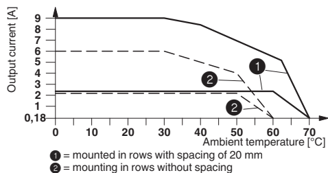
Derating curve ELR H3-IES-SC-230AC/500AC-2 and ELR H3-IES-SC-230AC/500AC-9
