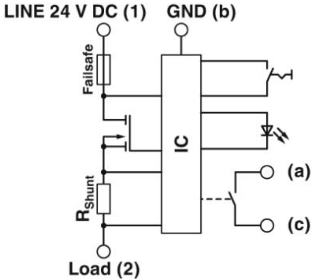
Circuit diagram
