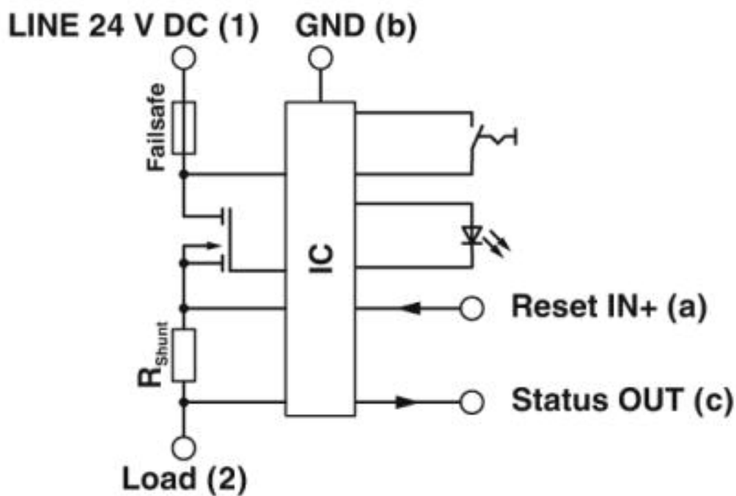
Circuit diagram
