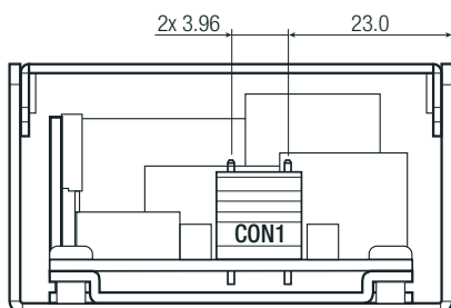
AC side
