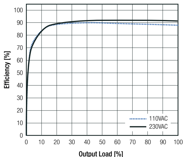
12V model
