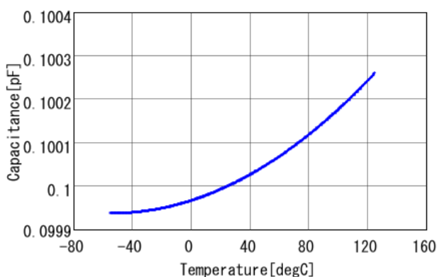
Tempetature Characteristics
