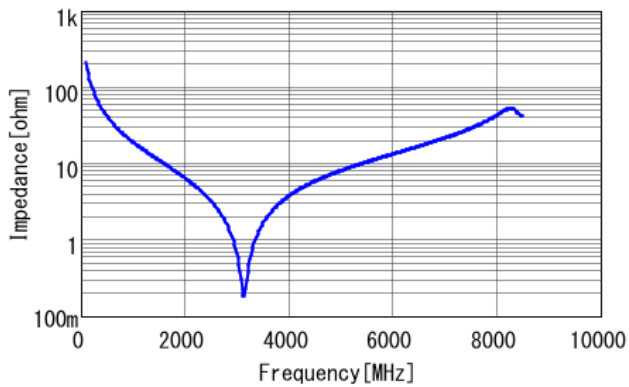
Frequency Characteristic|Z|
