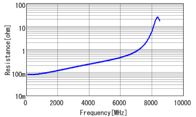
Frequency CharacteristicR
