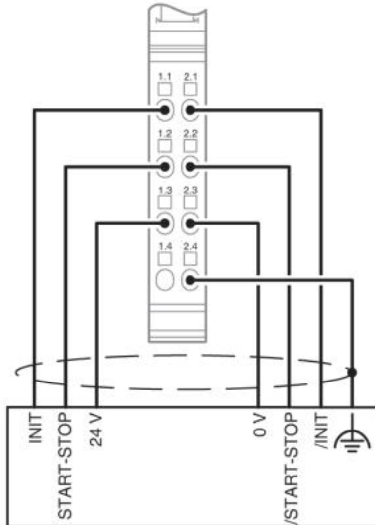
Connection diagram
