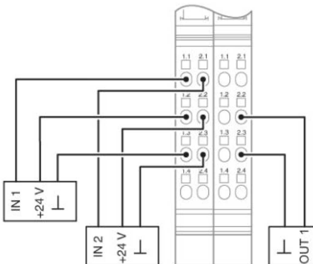
Connection diagram
