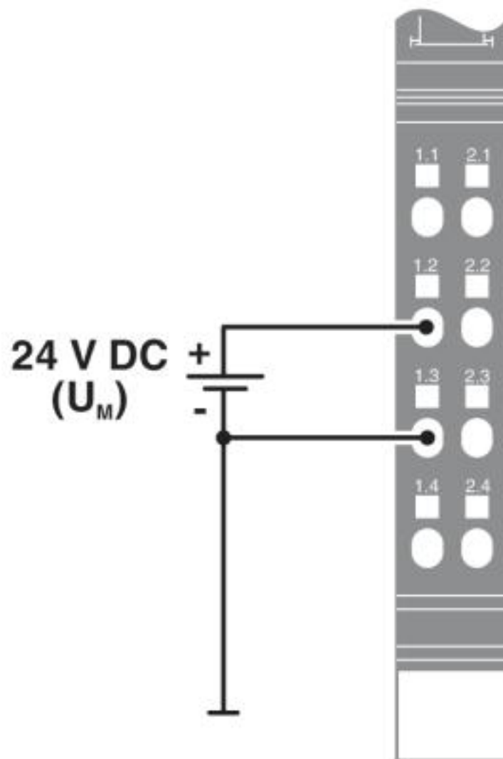
Connection diagram
