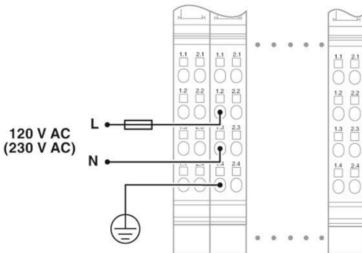
Connection diagram
