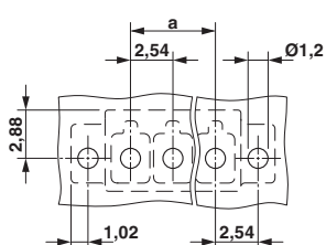
Drilling diagram
