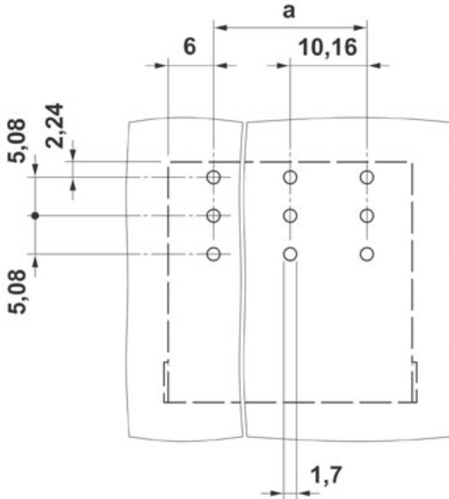
Drilling diagram
