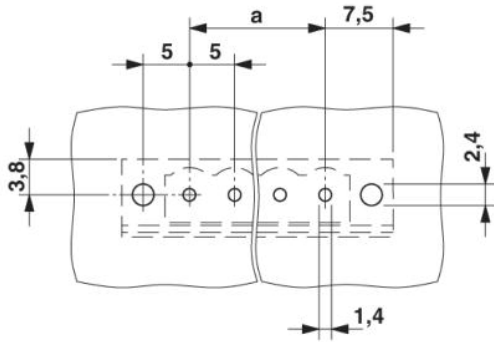
Drilling diagram
