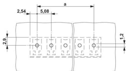
Drilling diagram
