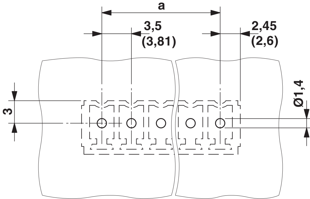
Drilling diagram
