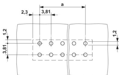
Drilling diagram
