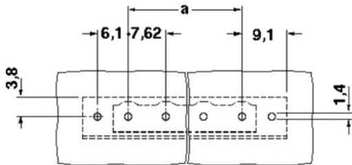
Dimensioned drawing
