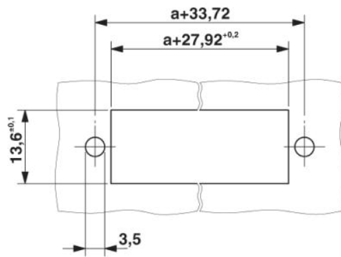
Sheet metal cutout for screw connection.
