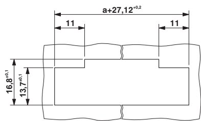
Dimensional drawing
