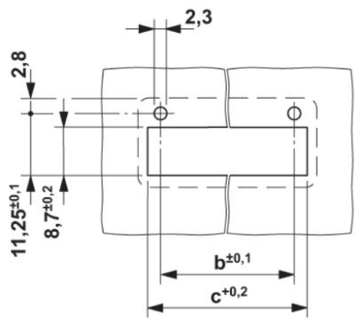
Drilling diagram
