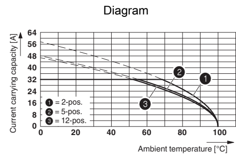
Derating curve for: IPC 5/...-ST-7,62 with IPC 5/...-G-7,62 Conductor cross section 6 mm 2
