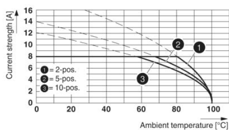
Type: TFMC 1,5/...-ST-3,5 with MC 1,5/...-G-3,5
