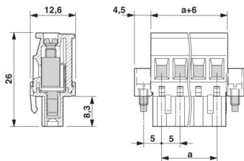
Dimensioned drawing
