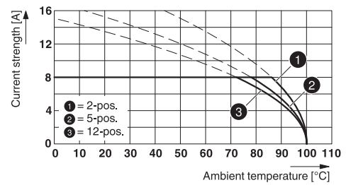
Type: FRONT-MC 1,5/...-ST-3,81 with MCV 1,5/...-G-3,81 P...THR
