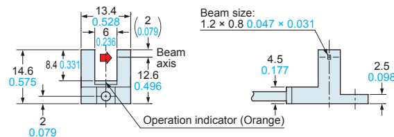
Sensor
