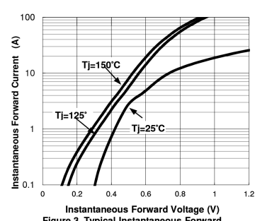
Figure 3. Typical Instantaneous Forward Characteristics Per Leg
