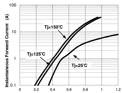
Figure 3. Typical Instantaneous Forward Characteristics Per Leg
