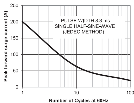
Figure 2. Maximum NON-Repetitive Surge
