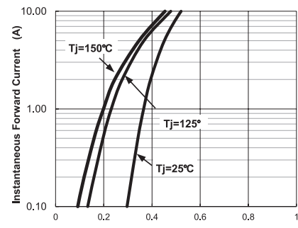
Figure 3. Typical Instantaneous Forward Characteristics Per Leg
