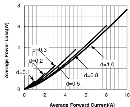
Figure 6. Forward Power Loss Characteristics
