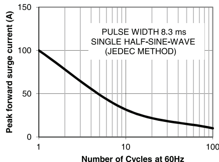
Figure 2. Maximum NON-Repetitive
