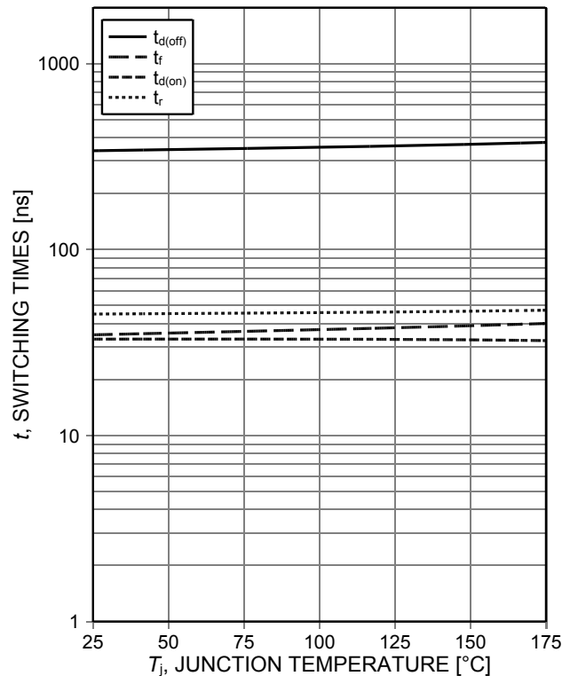
Figure 10. Typical switching times as a function of junction temperature (ind. load, V_{CE}=400\text{V} , V_{GE}=0/15\text{V} , I_C=75\text{A} , r_G=5\Omega , test circuit in Fig. E)
