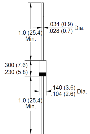
DO-204AC (DO-15)
