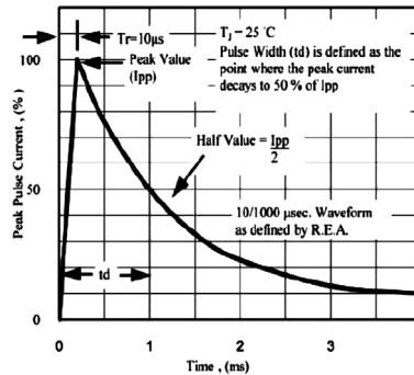
Fig. 5 - Pulse Waveform
