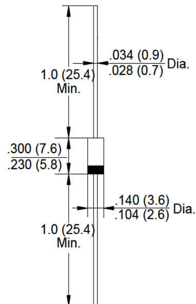
DO-204AC (DO-15)
