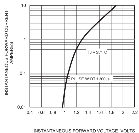
FIG.4-TYPICAL FORWARD CHARACTERISTICS
