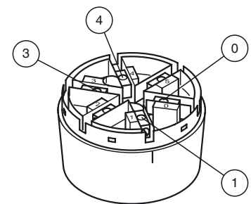
As AS-Interface signal tower
