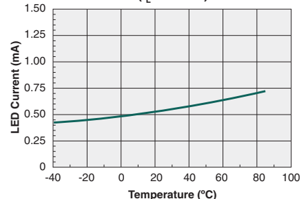
Typical I_F for Switch Dropout vs. Temperature ( I_L=100\text{mA} )
