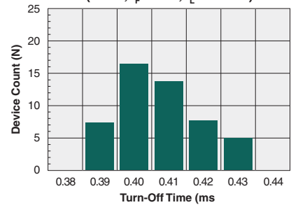
Typical Turn-Off Time (N=50, I_F=3\text{mA} , I_L=100\text{mA} )
