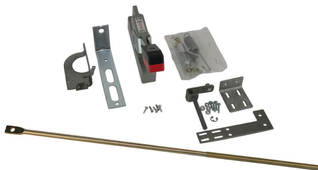
Flange rod operator kit for 30, 60 and 100 A switches.
