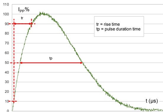
Figure 2. Pulse definition for electrical characteristics
