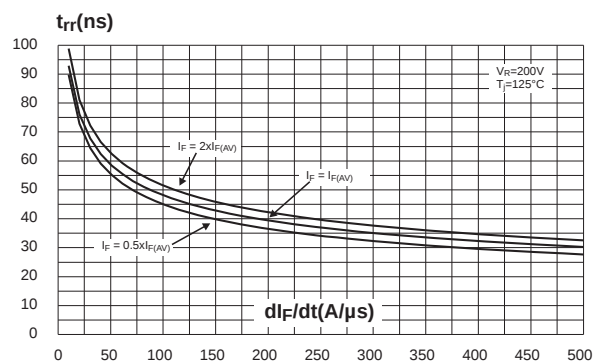
Figure 3. Reverse recovery time versus di_F/dt (typical values)
