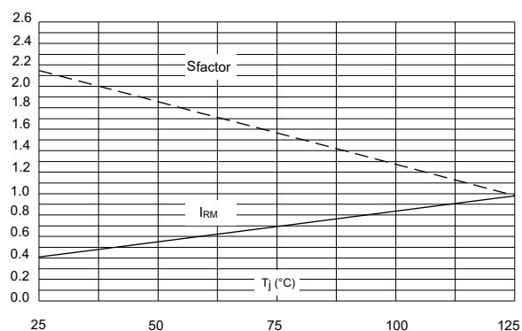
Figure 5. Relative variations of dynamic parameters versus junction temperature (reference: T_J = 125 °C)
