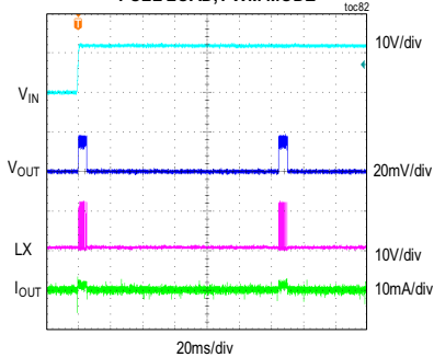
MAXM17904 OUTPUT SHORT DURING STARTUP V_{IN} = 12V , FIXED V_{OUT} = 3.3V , FULL LOAD, PWM MODE
