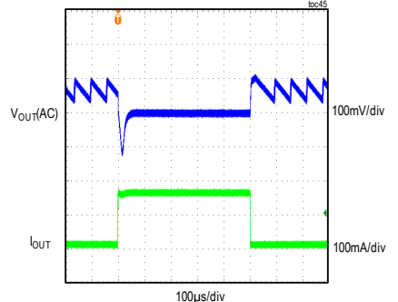
MAXM17906 LOAD TRANSIENT RESPONSE V_{IN} = 12V , ADJUSTABLE V_{OUT} = 3.3V , PFM MODE (LOAD CURRENT STEPPED FROM 5mA TO 150mA)
