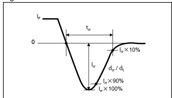
Fig.5-2 di/dt Waveform
