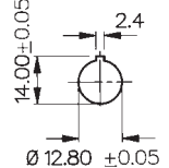
Fixing Details
