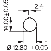
Fixing Details
