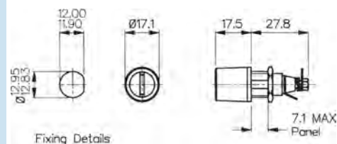
Fixing Details
