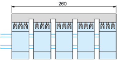
Sets of busbars GV2G345 and GV2G354
