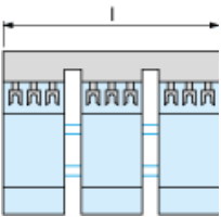
Sets of busbars GV2G345 and GV2G354
